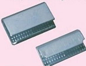
SUPER X4 and X5 12mm wide x 30mm long and 15mm wide x 30mm long. Indentations inside for a stronger seal. Open flanged for easy application. Thickness 0.7mm (12mm) and 1mm (15mm). Zinc finish. 1000 per pack.
