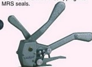
No 78 PP BUNDLER Crimper/tensioner combination. The easy and effective way to bundle pipes, garden stakes, timber etc. Simply insert the seal, lace the strap through it, tension as required, then depress the crimping/cutting lever. Use 12mm PP strapping with MRS seals.
