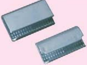
SUPER X4 and X5 12mm wide x 30mm long and 15mm wide x 30mm long. Indentations inside for a stronger seal. Open flanged for easy application. Thickness 0.7mm (12mm) and 1mm (15mm). Zinc finish. 1000 per pack.
